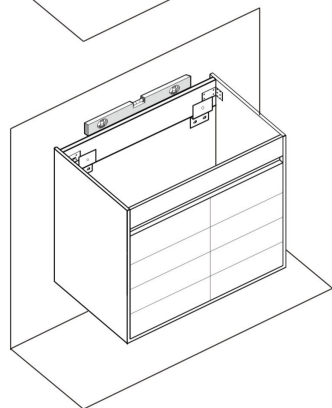
Marking hole position
